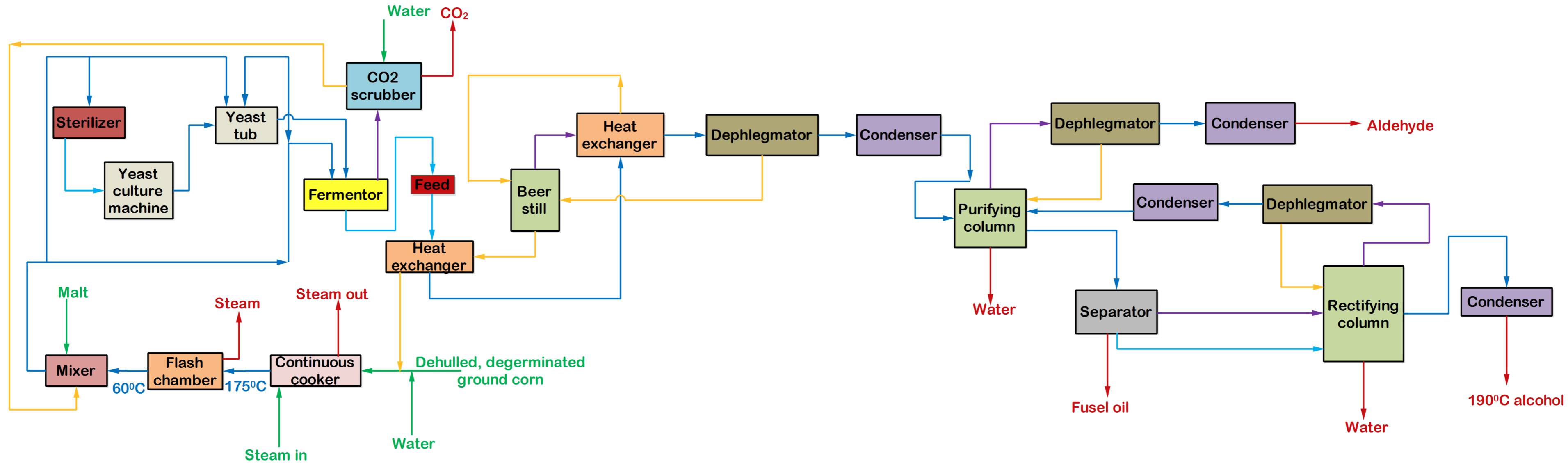
Figure: Manufacture of Industrial alcohol by malt fermentation
